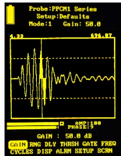
Pitch-Catch RF
