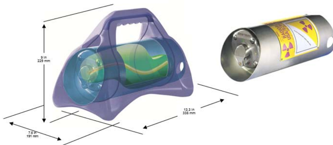
Figure 1 - 880 Configuration Views
