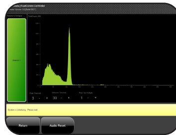
Cesium-137 Spectra
