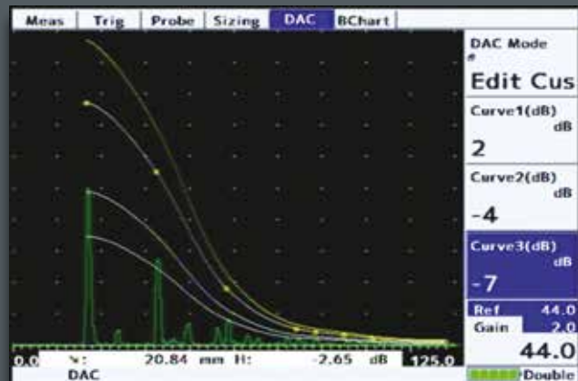
Customisable DAC
