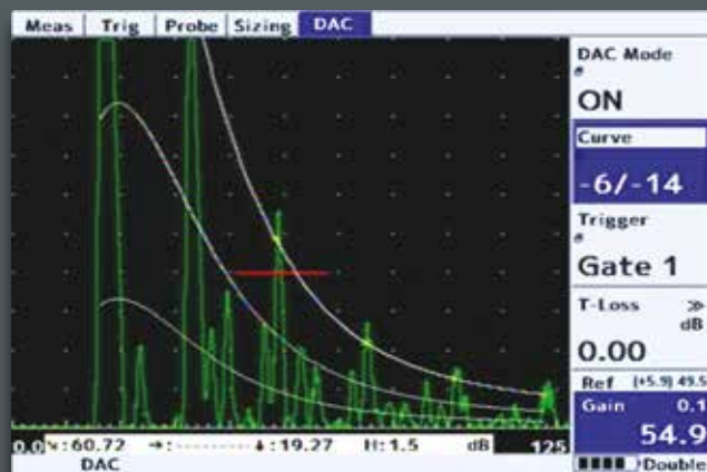
Dynamic DAC
